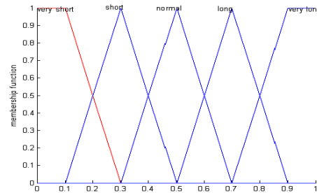
Figure 4. Membership Function of Dead Line Distance
