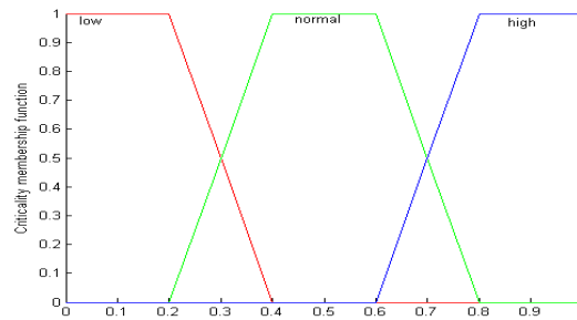
Figure 5. Membership Function of Fuzzy Scheduling priority.
